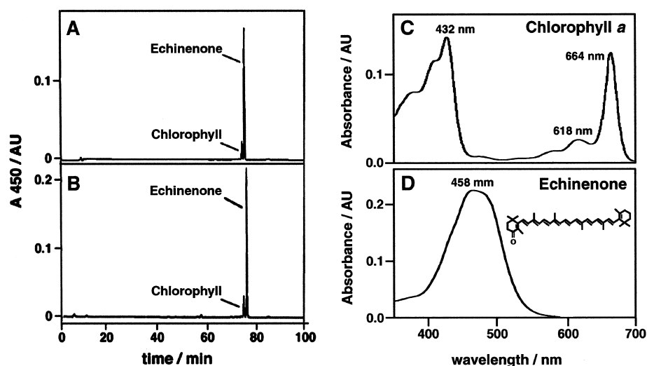
Fig. 3. Pigment analysis of the isolated cyt b_6f complex and the purified cyt b_6 subunit by reversed-phase HPLC. Column: Crom Spherisorb ODS 2, flow rate 0.5–0.9 ml/min at RT. Pigments were eluted by stepwise addition of ethyl acetate (buffer 2) to buffer 1 (38.5% (v/v) acetone, 46.5% (v/v) methanol, 5% (v/v) H_2O , 10% (v/v) 5 mM PIC A). (A) Elution profile of an acetonic extract from the isolated cyt b_6f complex (starting material for the cyt b_6 isolation). (B) Elution profile of an acetonic extract from the isolated cyt b_6 protein. (C) Absorbance spectra of chlorophyll a and (D) of echinenone, both recorded online from the peak fractions of run B.
